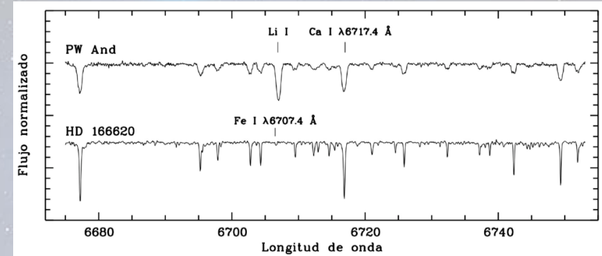
Li I line at 6707.76 Å In the spectrum of a young star ( López-Santiago et al, 2003 )
