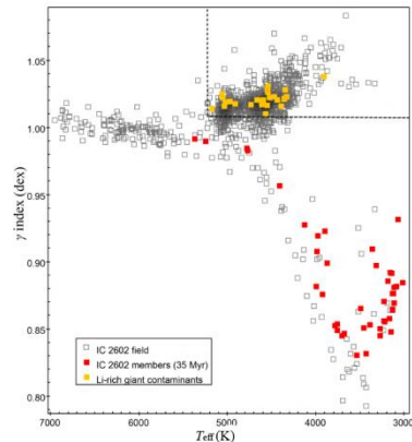
4) Gravity indicators: Kiel diagram and (\gamma, T_{\text{eff}}) plane
