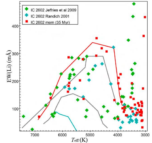
6) Position in EW(Li) vs T_{\text{eff}} diagram with empirical envelopes as guide.
