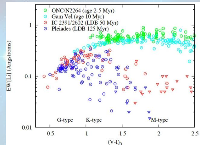
EW(Li) as a function of colour and spectral type for several clusters, from Soderblom et al. (2014) .
